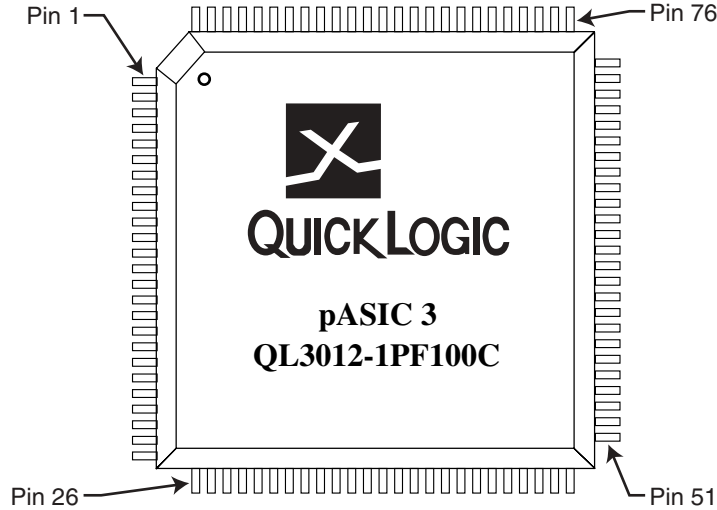
Figure 17: QL3012 – 100 Pin TQFP (Top View)
