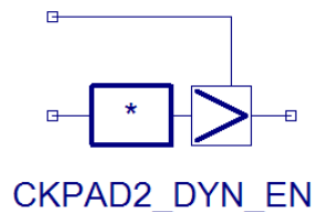
Figure 13: Clock Pad Macro for Dynamic Clock Enable
