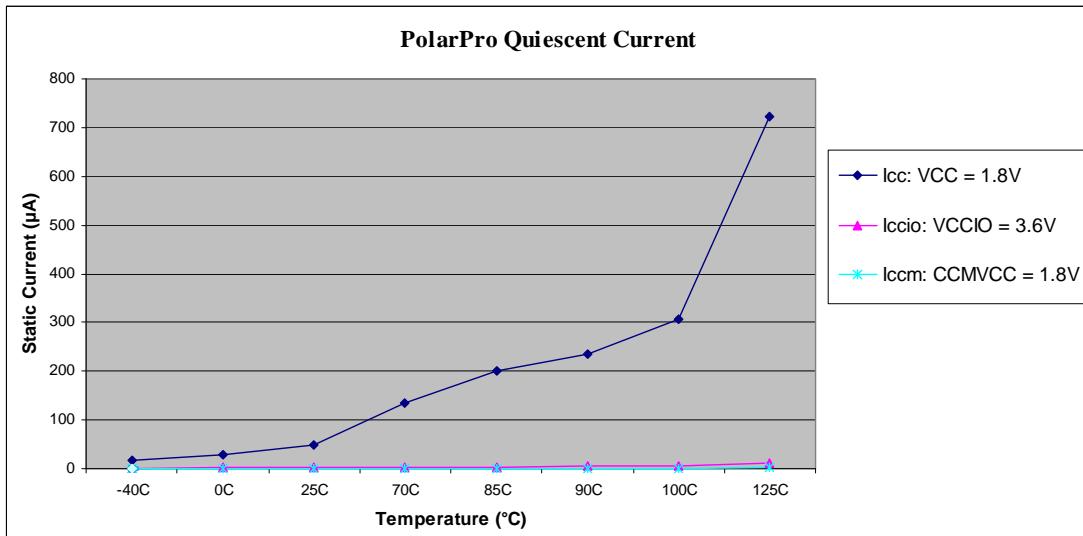
Figure 8: Quiescent Current for QL1P300 with VLP = 3.3 V
