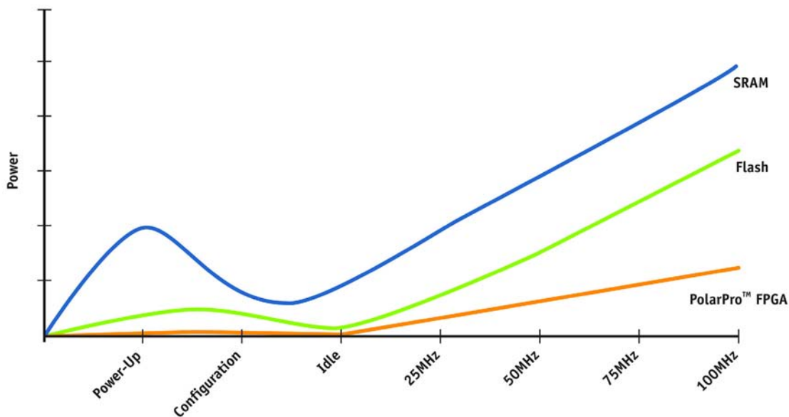
Figure 1: FPGAs Built Using Nonvolatile Memories Consume Far Less Power than SRAM-Based Devices
