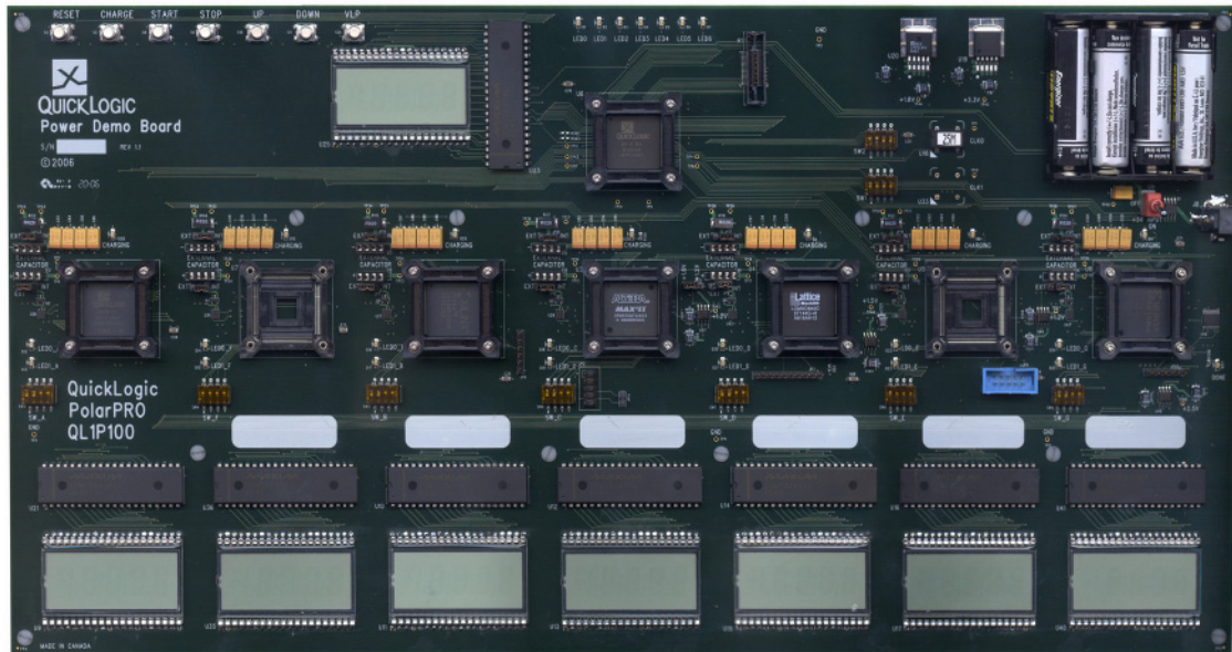
Figure 2: QuickLogic's Power Demo Board Provides a Visual Indication of FPGA Core Current Consumption
