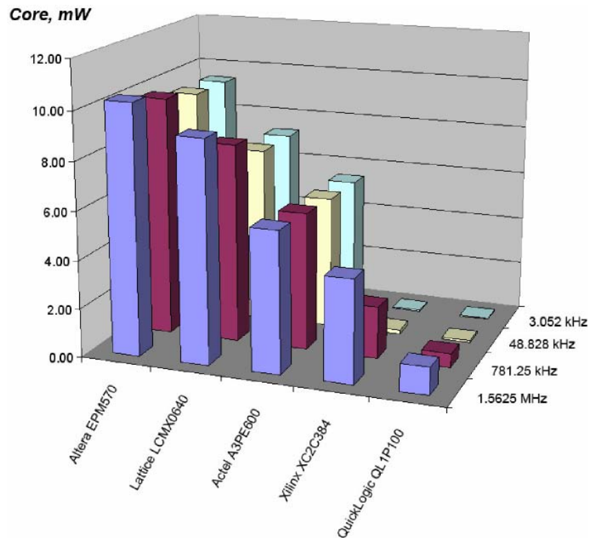
Figure 4: Core Power Consumption in mW at Four Test Frequencies 1
