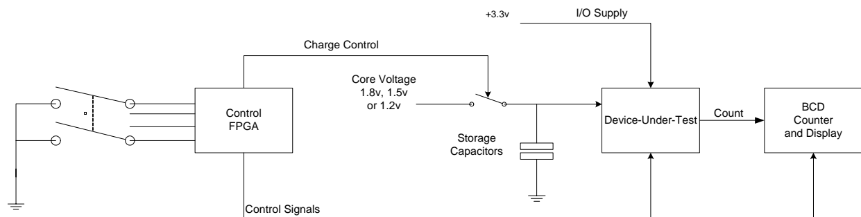
Figure 3: A Charge Counter Provides a Visual Indication of a DUT's Power Drain
