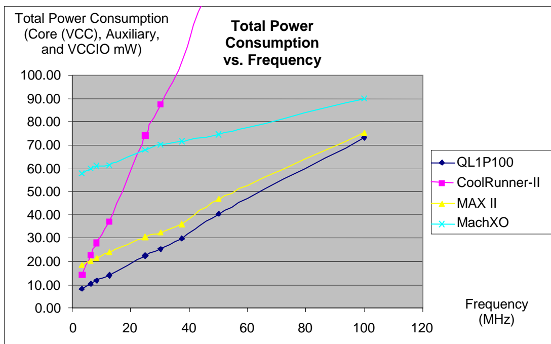
Figure 5: Total FPGA Power Drain Strongly Depends on Clock Frequency
