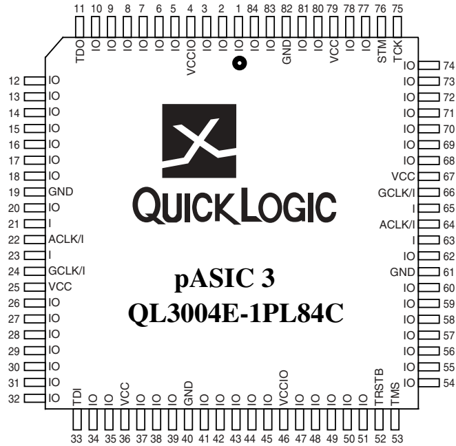
Figure 11: QL3004E – 84 Pin PLCC (Top View)
